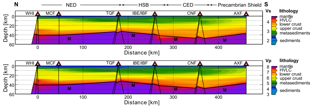
Figure 10. S -wave model results (middle panel) and P -wave model results (lower panel) interpolated between each BAZ bin and projected along the average ray path (black lines). M—Moho interpretation. White shading—interpolated areas without data coverage ( \sim 15 km surrounding each ray path).
